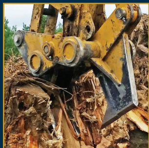
Ransome RSH40 Mechanical Splitter
